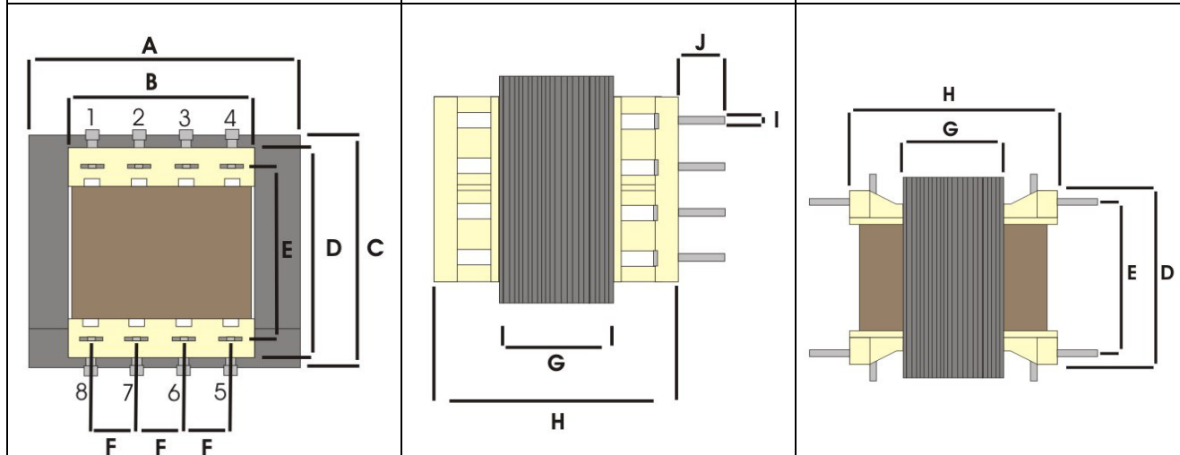
VISTA FRONTAL
