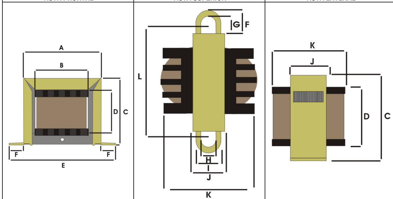
VISTA FRONTAL
